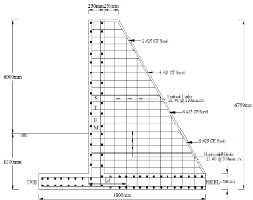
CROSS SECTION THROUGH THE COUNTERFOOT
