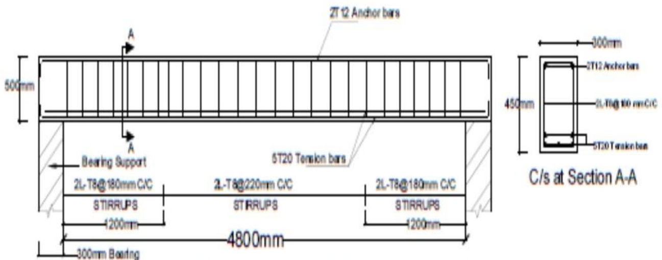
L/S OF SIMPLY SUPPORTED SINGLY REINFORCED BEAM
